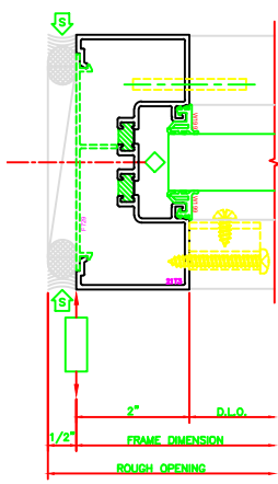
401 I.G. JAMB SERIES 400X - 2" X 4 1/2" SHEARBLOCK
